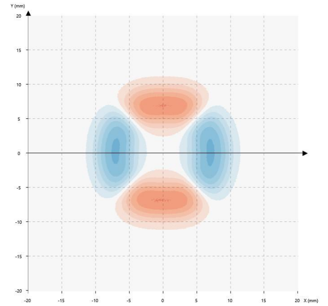
Ring with axial 4 poles
