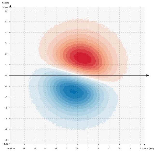
Disc with axial 2 poles
