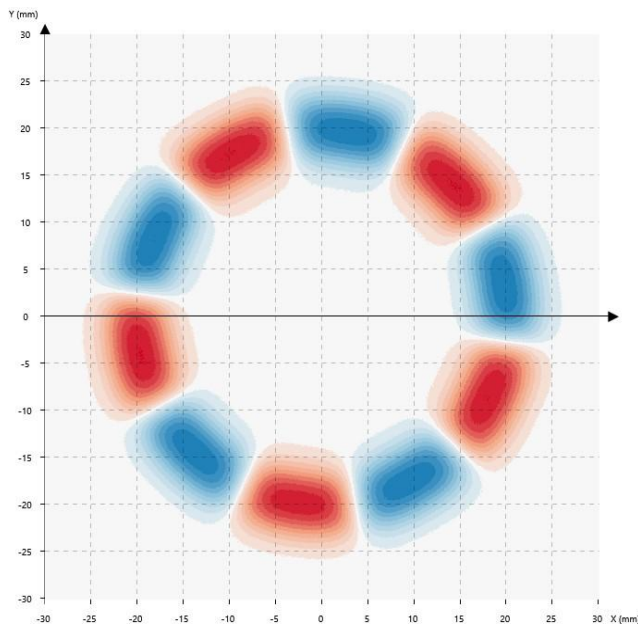
Ring with axial 10 poles
