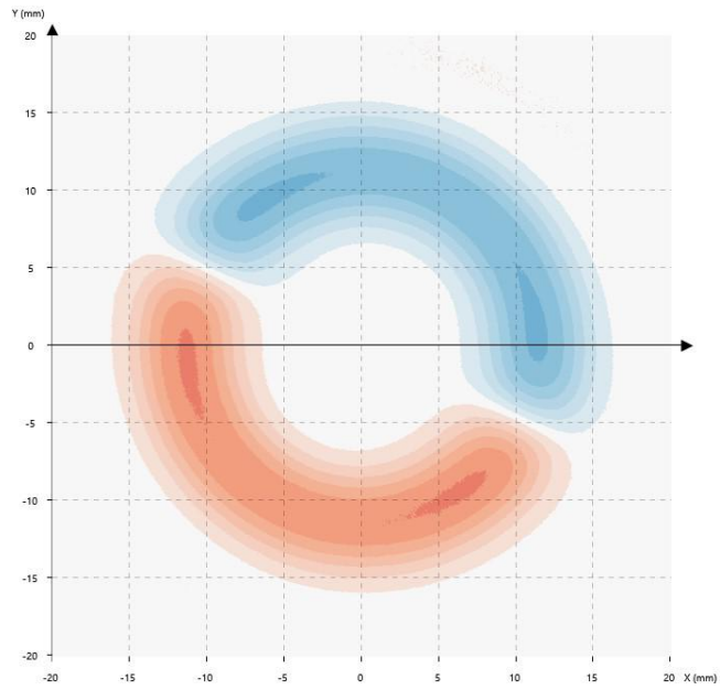
Ring with axial 2 poles
